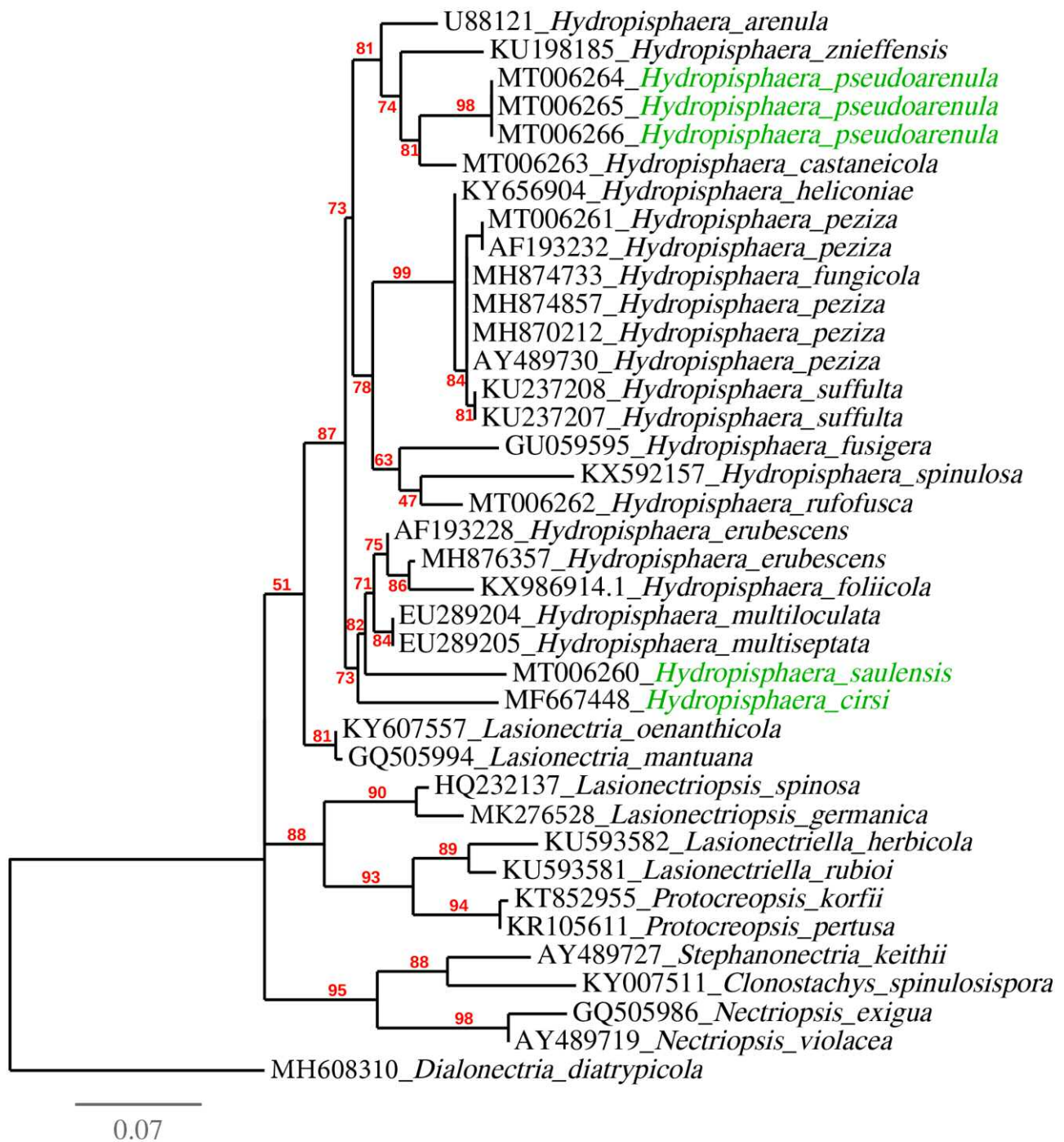
Fig. 1 – Maximum likelihood phylogeny ( -\ln L = 2025.63218 ) of Hydropisphaera spp. inferred by PhyML 3.0, model HKY85 from a 820 bp matrix of 28S rRNA sequence, rooted with Dialonectria diatrypicola .
