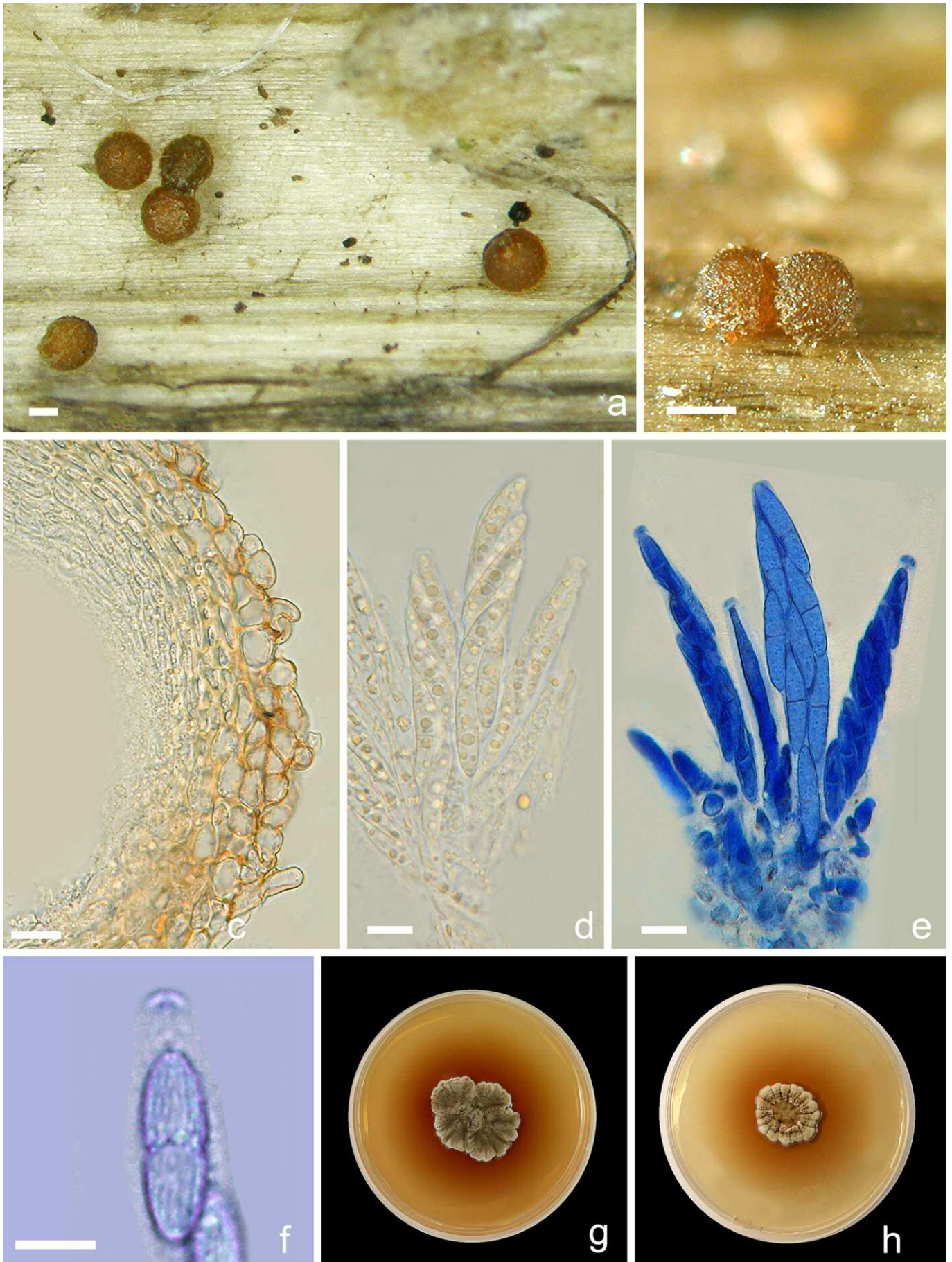
Fig. 3 – a-e, g, h: Hydropisphaera pseudoarenula ; a: Ascomata on the substrate; b: Close-up of ascomata in natural environment; c: Vertical section through lateral ascumatal wall; d: Asci and ascospores in water; e: Asci and ascospores in lactic cotton blue; f: H. arenula (JF08061), tip of ascus and striate ascospore (in dilute blue ink); g, h: Cultures at three weeks; g: CLL19020, h: CLL11052. Scale bars: a = 100 \mu m; b = 200 \mu m; c-e = 10 \mu m; f = 5 \mu m.
